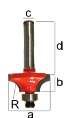
BEADING BIT
